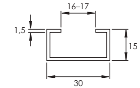
C-rail dimensions (mm)
