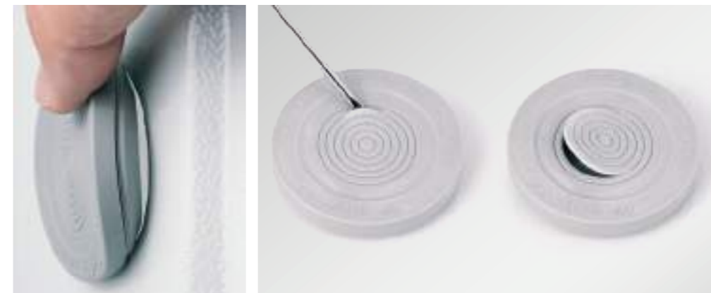
The single membrane rings are peeled off according to the diameter of the routed cable or hose. For this purpose, only a small hole between the rings needs to be pierced. Then the corresponding ring can be removed.
